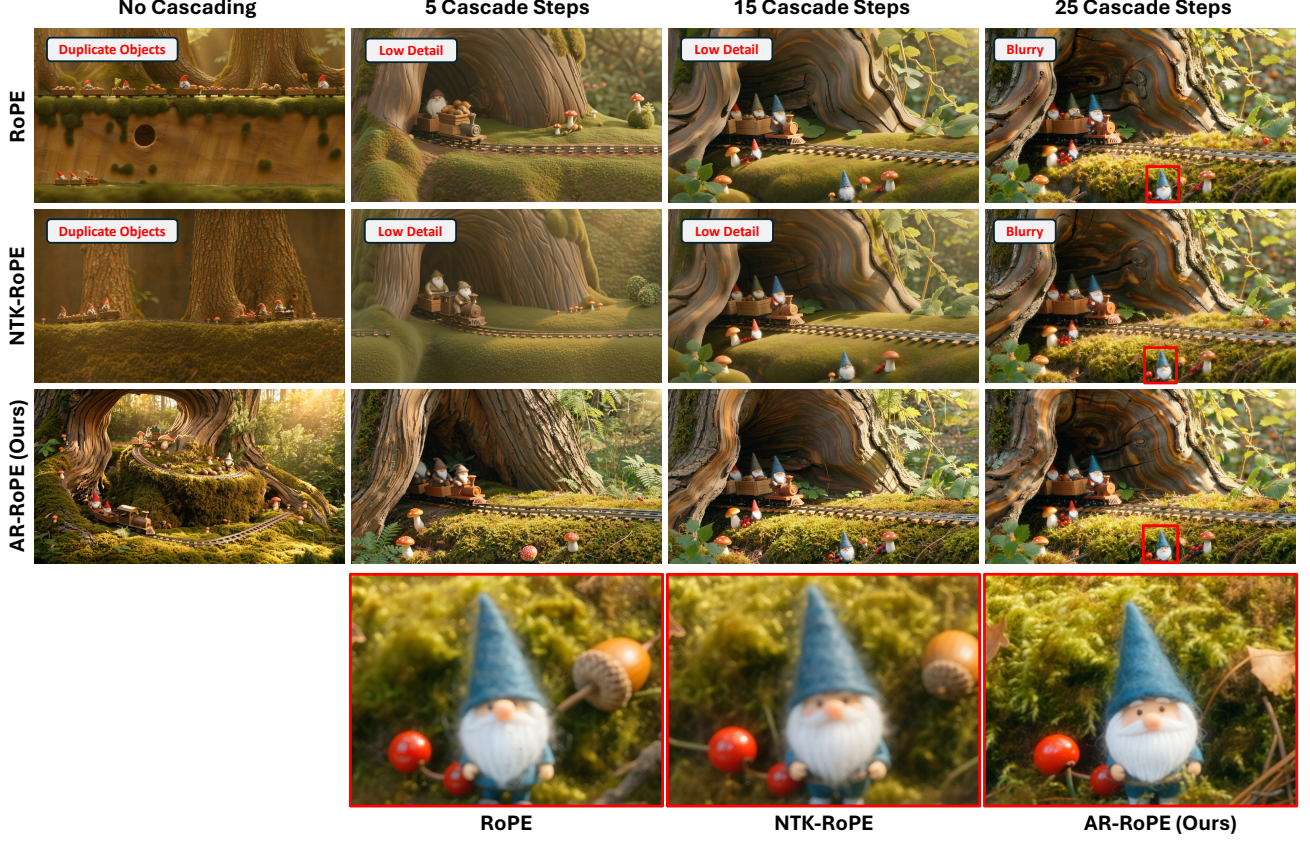
Figure 6. Ablation of RoPE variants at 4K resolution. Standard RoPE and NTK-RoPE produce structural artifacts under large spatial extrapolation and yields over-smoothed details and jittering. Adaptively Rectified RoPE preserves local positional geometry while rectifying distant offsets, resulting in sharper details and more coherent global structure.
