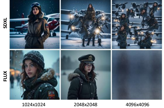
Figure 4. Distinct Failure Modes of U-Net and DiT Diffusion Models. Diffusion models built on U-Nets suffer from low receptive field resulting in global incoherence while those built on DiTs suffer out-of-distribution position encodings resulting in blurring.
