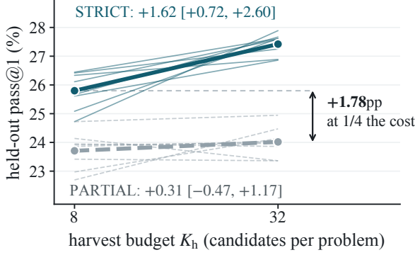
Figure 2: Search is a multiplier, not a substitute. Held-out pass@1 for the four count-matched APPS arms, as means over eight training seeds on 150 held-out problems; thin lines are the individual seeds. Every contrast is paired by seed.
