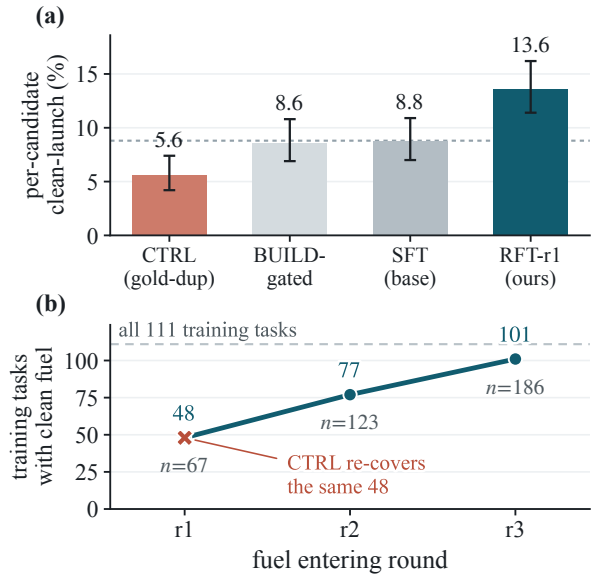
Figure 3: (a) Same 67-sample budget; the dashed line is the supervised model’s rate. Neither control improves on it: exact gold duplication regresses ( p = 0.018 ) and the lenient BUILD filter merely matches it. Only STRICT-LAUNCH-filtered self-distillation gains ( p < 10^{-4} against CTRL, p = 0.0012 against BUILD-gated). (b) What the precise gate buys: the training tasks, of 111, whose fuel contains a clean project, with each round’s fuel size beside its point. The exact-duplication control re-covers the 48 that round 1’s fuel already reaches.
