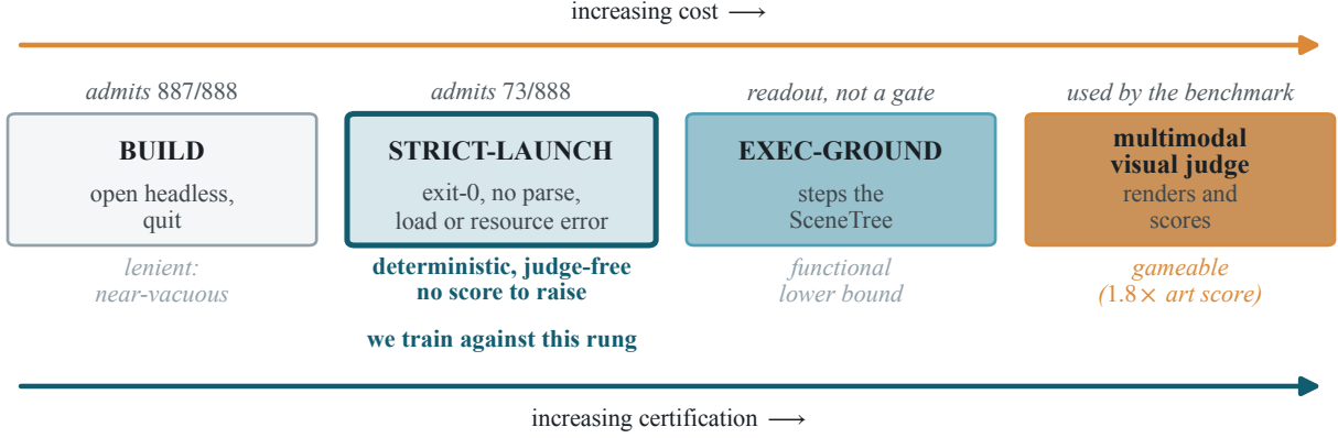
Figure 4: The verification ladder , ordered by how much each signal certifies. BUILD is near-vacuous (it admits 887 of the supervised model’s 888 training-family candidates, of which only 73 also pass STRICT-LAUNCH ); STRICT-LAUNCH , our training gate, requires a clean headless launch (exit code 0, no parse/load/resource error), deterministic and judge-free; execution grounding drives the running SceneTree and serves as a readout rather than a gate; the top rung, a multimodal visual judge, certifies the most but is gameable.
