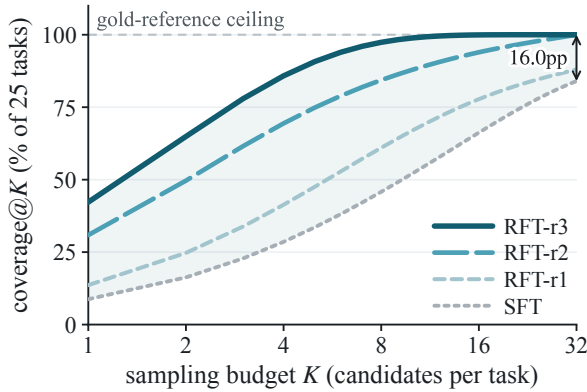
Figure 7: The supervised model never closes the coverage gap within the sampled budget. Coverage@ K under the unbiased estimator 1 - \frac{n-c}{\binom{n}{K}} , pooling four decoding seeds into n=32 candidates per task, c of them clean, averaged over the 25 held-out tasks. The supervised model is still 16.0pp short of full coverage at K=32 ; round 3 has been above 97% since K=8 .
