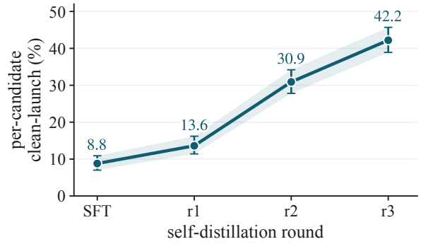
Figure 8: Three rounds compound. The per-candidate clean-launch rate on the four held-out families climbs 8.8 \rightarrow 13.6 \rightarrow 30.9 \rightarrow 42.2\% with Wilson intervals. Task-level coverage is not co-plotted; at the full 32-candidate budget it runs 84 \rightarrow 88 \rightarrow 100 \rightarrow 100\% , saturating at round 2. This series is the single-run trajectory the matched controls are compared against; the three-seed means are in Table 1.
