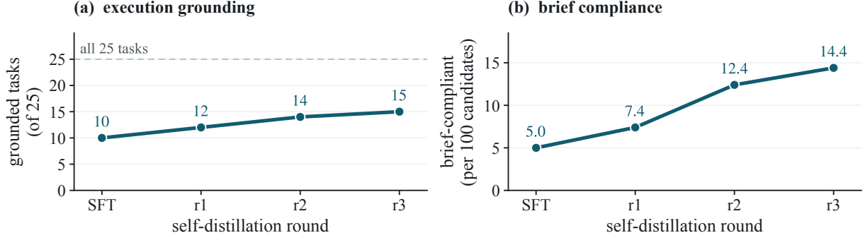
Figure 6: Two readouts the gate never optimizes. (a) Execution grounding: tasks with at least one grounded ( \geq 0.50 ) clean candidate, 10 \rightarrow 12 \rightarrow 14 \rightarrow 15 of the same 25 held-out tasks; the score is validated by 15/15 grounded gold against 0/16 known-bad projects. (b) Brief compliance under a blind judge that reads only the brief and the shipped GDScript: projects per 100 candidates that both launch and implement their brief.
