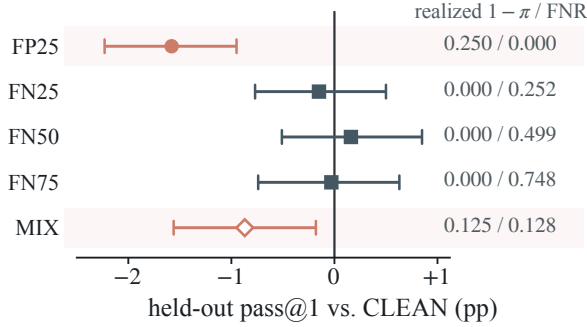
Figure 5: Only one direction of verifier error is paid for. Held-out pass@1 relative to the CLEAN arm on APPS, in percentage points, with 95% crossed seed × task bootstrap intervals, at a common count-matched quota over eight training seeds. Realized, not nominal: 1 - \pi is the non-all-pass share of the admitted rows (the axis of Fig. 1); the FNR is masked true positives over those available. FN arms mask true positives, FP25 injects false ones, MIX splits the error budget evenly.
