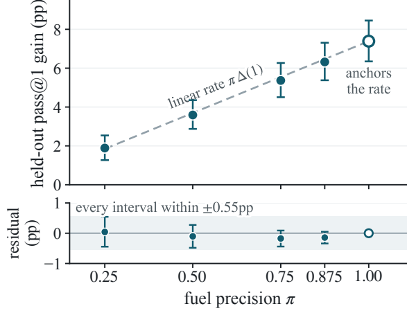
Figure 1: Linear conversion of clean fuel into transfer. Held-out gain over M_0 (pp) against fuel precision \pi , the fraction of the admitted candidates that pass all tests. The APPS arms are controlled : \pi is set by construction at fixed task set, gold pool, and candidate count (1300). Dashed: the linear rate \pi \Delta(1) , where \Delta(1) is the gain from clean fuel. Lower panel: residuals from that rate. Bars are 95% crossed seed \times task bootstrap CIs over 23 training seeds and 470 problems.
