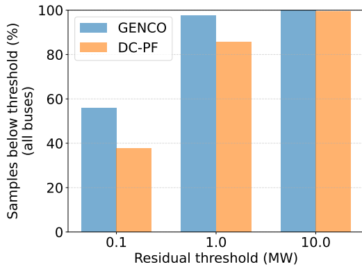
Figure 23. Percentage of samples below absolute active power-balance residual thresholds at k = 10 (all buses). GENCO again dominates DC-PF across all thresholds.
