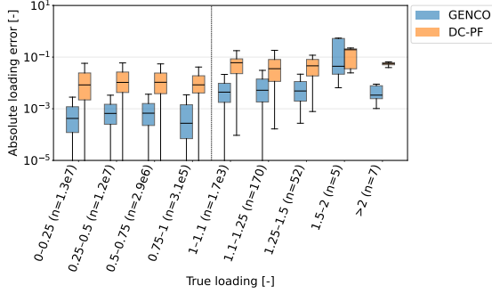
Figure 14. Absolute branch loading prediction error as a function of the true loading level. n indicates the number of test samples in each bin.
