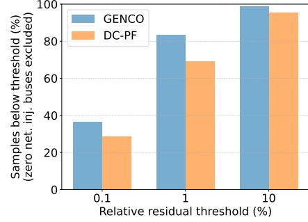
Figure 12. Percentage of samples below relative active power-balance residual thresholds at k = 10 (excluding zero net injection buses). GENCO achieves a larger share of low-residual predictions than DC-PF across all reported thresholds.
