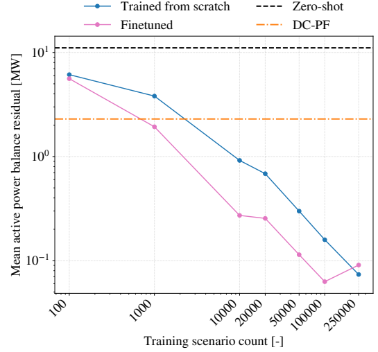
Figure 15. Mean active power-balance residuals on IEEE 118 for fine-tuned pretrained models and models trained from scratch using datasets of varying size. DC-PF and the zero-shot pretrained model (without fine-tuning) are shown as baselines.
