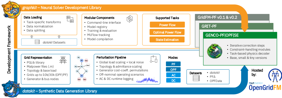
Figure 1. Representation of GENCO , our GEometric Neural Corrective Optimizer, within the GridFM development framework composed of gridfm-graphkit for neural solver training and evaluation, and gridfm-datakit for synthetic data generation. All three are released within the Linux Foundation for Energy OpenGridFM project and are available on GitHub . All datasets are available on Hugging Face .
