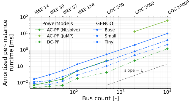
Figure 8. Amortized per-instance runtime versus grid size for GENCO and PowerModels AC-PF and DC-PF at the best batch size or worker count. Scaling exponents fitted on the four largest grids (two for AC-PF) are comparable across all methods, ranging from 0.94 to 0.97.
