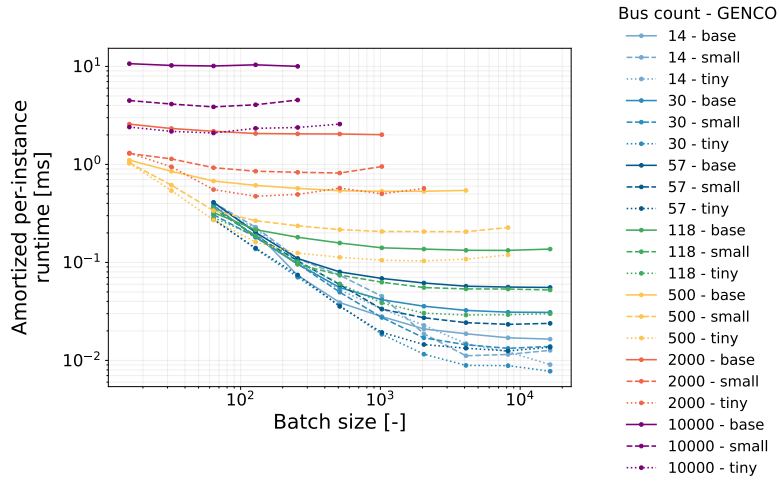
Figure 20. GENCO wall-clock time per instance versus batch size across grids and model scales.
