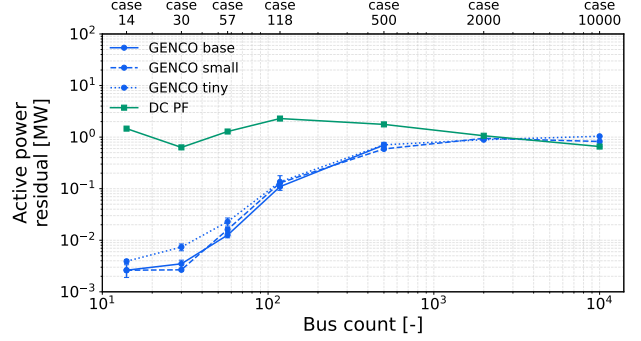
Figure 9. Mean active power-balance residuals versus grid size for GENCO and PowerModels DC-PF.
