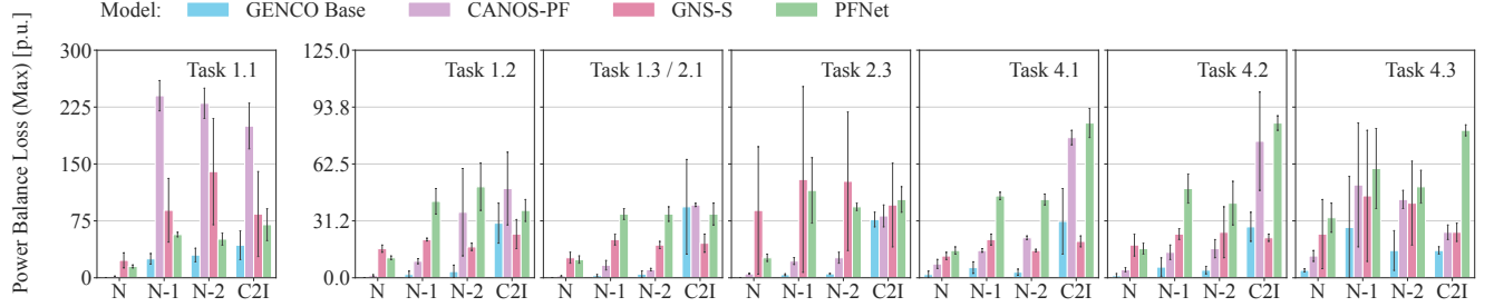
Figure 18. Max power-balance loss (computed across all buses of all samples) for GENCO, CANOS-PF, GNS-S, and PFNet across PF \Delta tasks on the IEEE 118-bus system. Error bars in the figure correspond to the standard deviation over three seeds. C2I denotes close-to-infeasible cases at the steady-state stability limit, where classical solvers face challenges [49].
