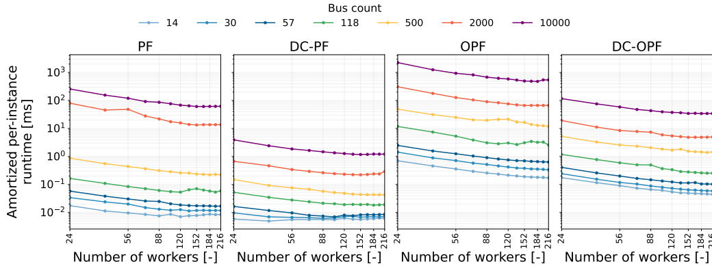
Figure 21. PowerModels wall-clock time per instance versus worker count for AC-PF, DC-PF, AC-OPF, and DC-OPF across grids using the in-memory protocol.
