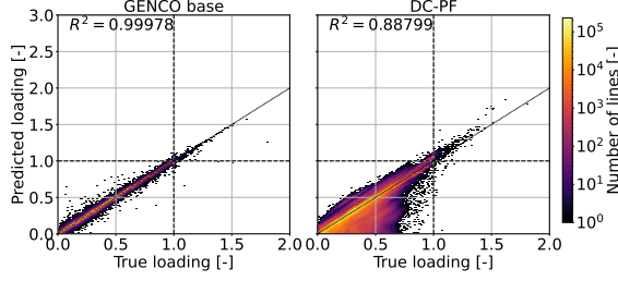
Figure 13. Relative branch loading predictions obtained with GENCO base (left) and DC-PF (right) compared to AC-PF loadings. Values above 1.0 indicate thermal overloads.
