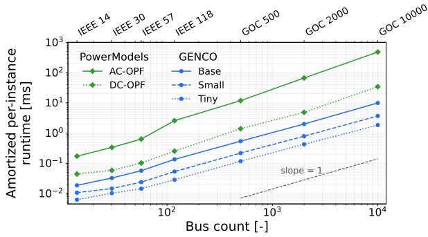
Figure 10. Amortized per-instance runtime versus grid size for GENCO and PowerModels AC-OPF and DC-OPF solvers. Results are reported for the optimal batch size for GENCO and the best worker count for PowerModels. Four-largest-grid scaling exponents are 1.18 for AC-OPF, 1.09 for DC-OPF, and 0.97/0.95/0.94 for GENCO Base/Small/Tiny.
