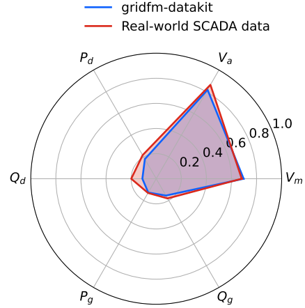
Figure 2. Normalized mean feature entropy of real-world SCADA PF data from HQ1200 and synthetic PF data generated for HQ1200 using gridfm-datakit. Values close to one indicate higher diversity, with one corresponding to a uniform distribution. Features are: V_m/V_a : bus voltage magnitudes/angles; P_g/Q_g : active/reactive power generation; P_d/Q_d : active/reactive power demand.
