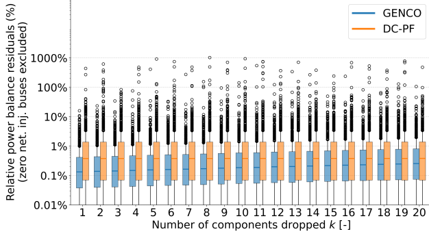
Figure 11. Bus-level active power-balance residuals (excluding zero net injection buses) for GENCO and DC-PF under N- k contingencies ( k = 1, \dots, 20 ) on the Texas 2000-bus system. GENCO is trained only on N-2 perturbations. Whiskers indicate 1.5 \times \text{IQR} .
