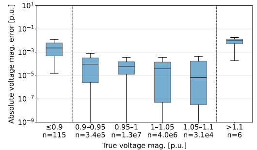
Figure 28. Absolute voltage magnitude prediction error as a function of the true voltage magnitude. n indicates the number of test samples in each bin.
