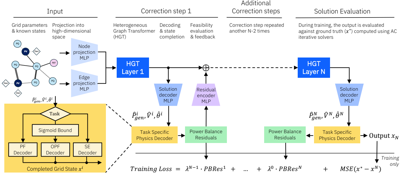
Figure 3. Overview of GENCO.
