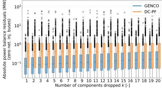
Figure 25. Bus-level absolute active power-balance residuals at zero-net-injection buses under N-k contingencies ( k = 1, \dots, 20 ). GENCO achieves consistently lower residuals than DC-PF across the entire distribution. Whiskers indicate 1.5 \times \text{IQR} .
