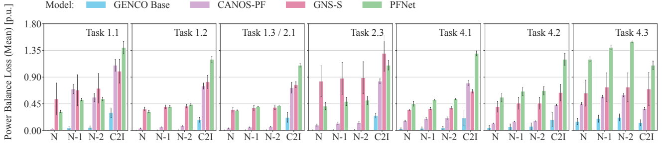
Figure 4. Mean power-balance loss (averaged across all buses of all samples) for GENCO, CANOS-PF, GNS-S, and PFNet across PF \Delta tasks on the IEEE 118-bus system. Error bars in the figure correspond to the standard deviation over three seeds. C2I denotes close-to-infeasible cases at the steady-state stability limit, where classical solvers face challenges [49].
