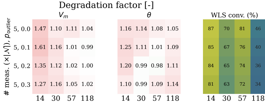
Figure 19. Degradation in scenarios where WLS did not converge (at a sparse coverage of 5|\mathcal{N}| measurements). The first two panels report, for V_m and \theta , the ratio of GENCO’s error on scenarios where the baseline did not converge to its error on scenarios where it did (rows sweep the outlier probability p_{\text{outlier}} ). Values near 1 mean GENCO is almost as accurate on the hard, non-converged cases as on the easy ones, i.e. it degrades gracefully rather than failing outright; values above 1 indicate higher error on the hard set. The last panel shows the WLS convergence rate. Columns are the IEEE 14-, 30-, 57-, and 118-bus grids.
