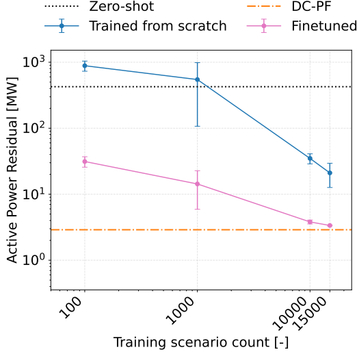
Figure 16. Mean active power-balance residuals on HQ SCADA versus number of training scenarios, comparing fine-tuning of the synthetically pretrained model against training from scratch (mean \pm sample std over three seeds). The dotted line denotes zero-shot performance of the pretrained model.
