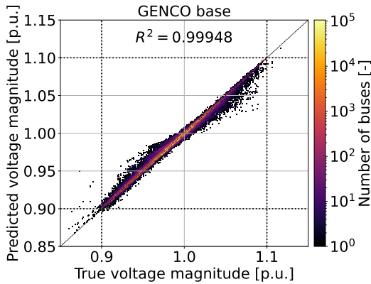
Figure 27. Bus voltage predictions obtained with GENCO compared to AC-PF voltages.
