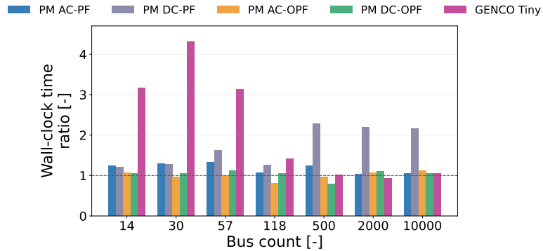
Figure 22. Ratio of loading-inclusive to in-memory wall-clock time per instance at the best configuration selected independently under each protocol. The dashed line marks equal time; values above one indicate loading overhead.
